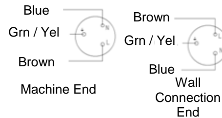
Detail for wire connections
